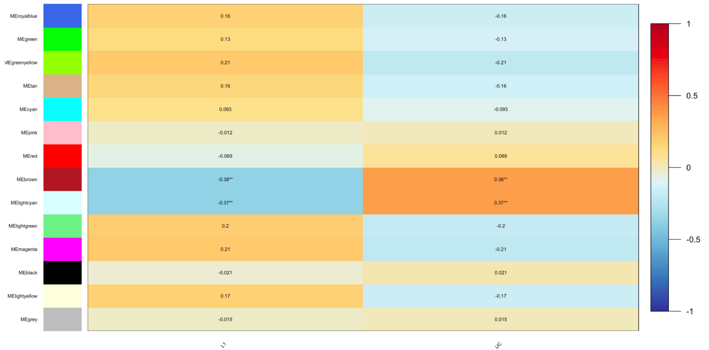
Module-trait relationships
